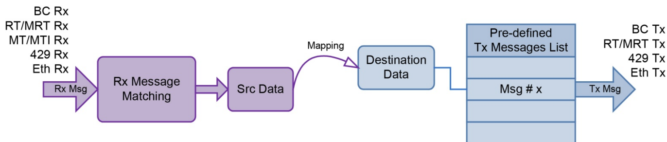
Figure 18. Protocol Conversion Layer Flow Diagram
