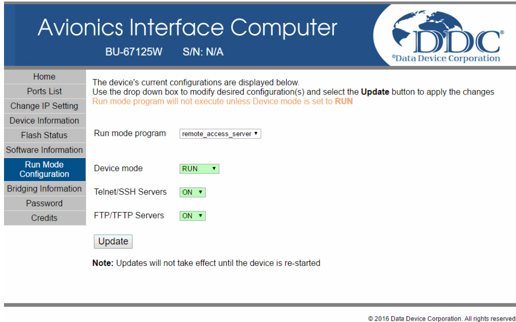
Figure 13. C-AIC Run Mode Configuration
