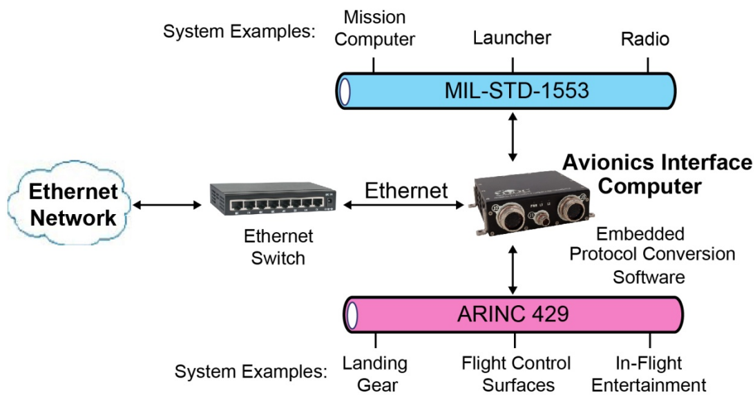
Figure 2. Example of the C-AIC in Protocol Conversion Mode
