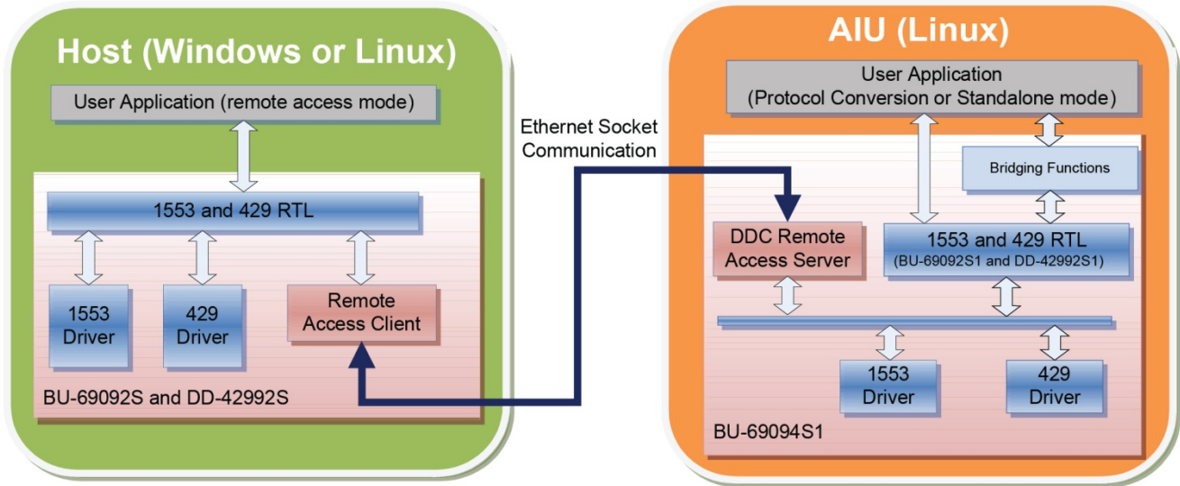
Figure 27. C-AIC Remote Access interaction
