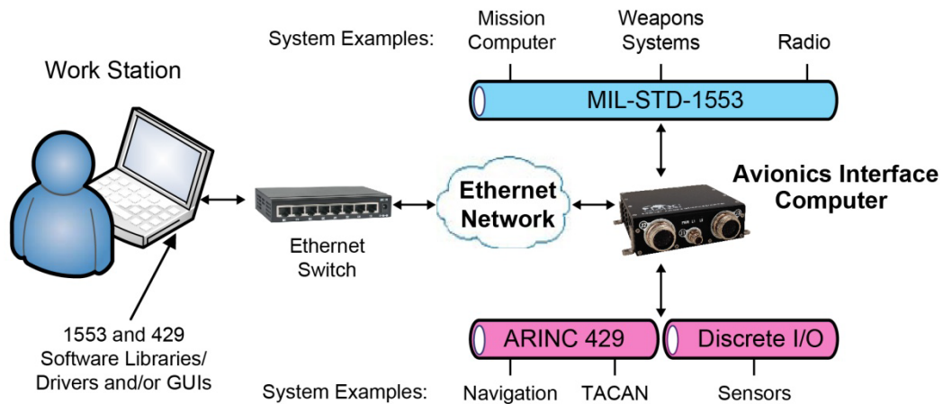
Figure 3. Example of the C-AIC Used in Remote Access Mode
