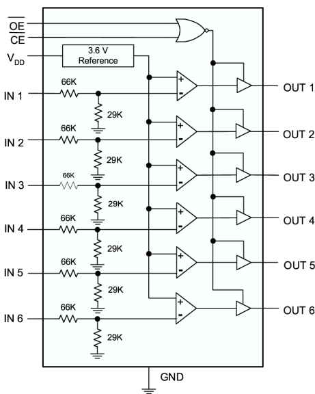
Figure 1: Function Diagram
