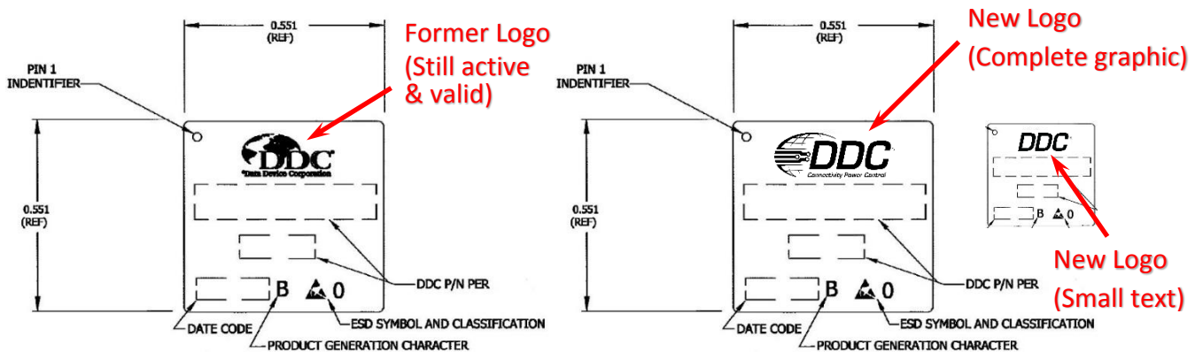
Figure 2 Generic Part Marking Drawing
